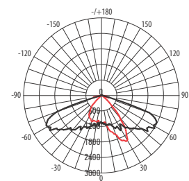
PSL 03 50W 5000K IP65
